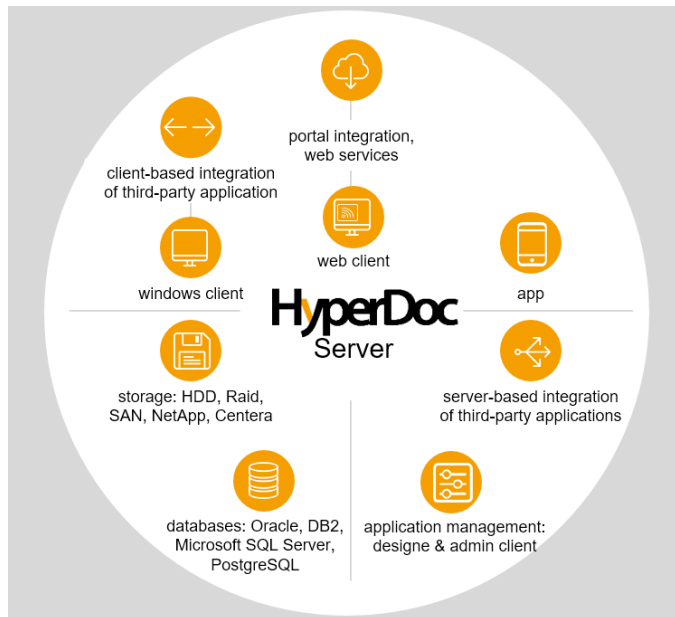
Fig.: HyperDoc architecture
